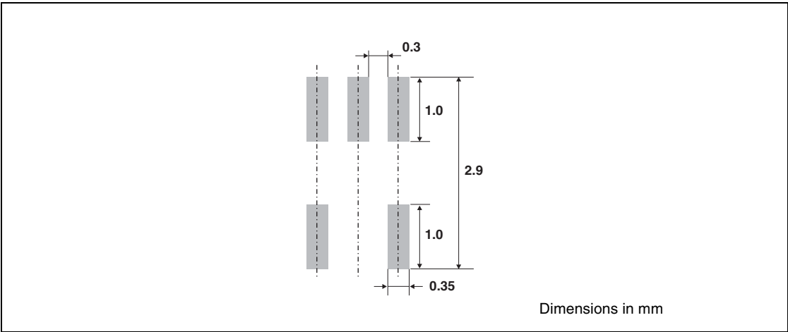
Figure 8. Footprint dimensions
